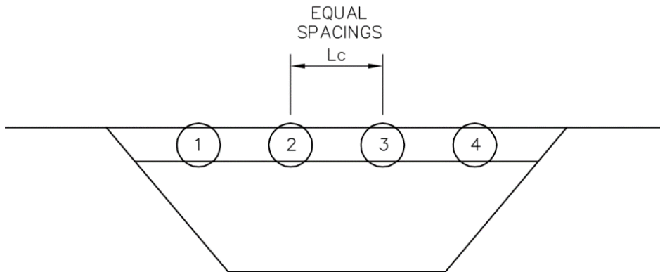
Figure 11.3.6.B - Horizontal Bridge
