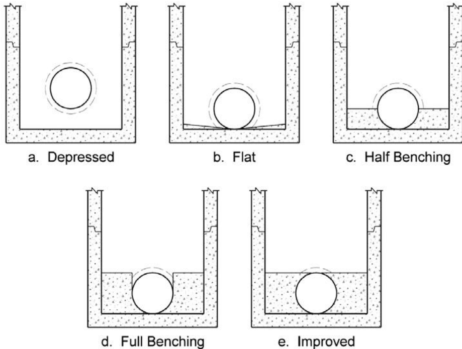
Figure 7.2.6.3.C - Manhole benching methods (Source FHWA HEC-22, 3 rd Edition)
