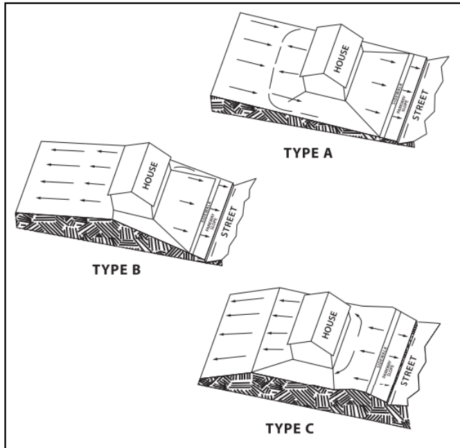
Figure 15.2 - Typical FHA Lot Grading
