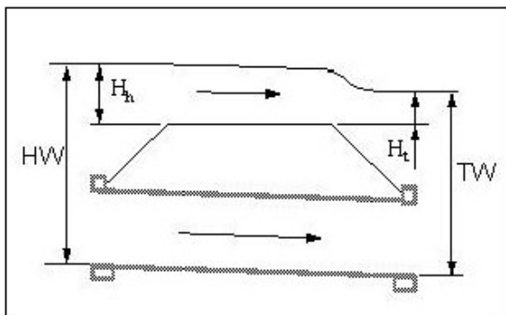
Figure 10.3.13.B - Over-Embarkment Flow Adjustment Factor (Source TxDOT, Hydraulic Design Manual, 2011)
