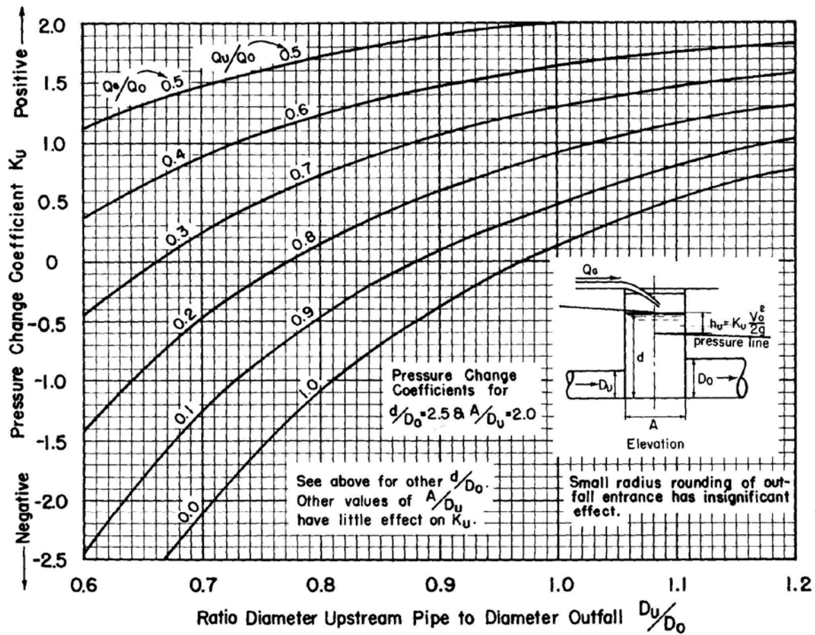
Figure B.4 Chart 4 - Rectangular Inlet With Through Pipeline And Grate Flow (Source University of Missouri E.S.B. #41)
