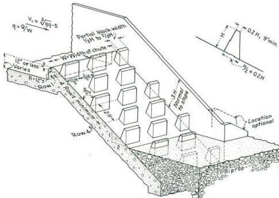
Figure 9.3.7 USBR Type IX Baffled Apron Peterka, 1978, (Source FHWA, HEC-14 Hydraulic Design of Energy Dissipators)
