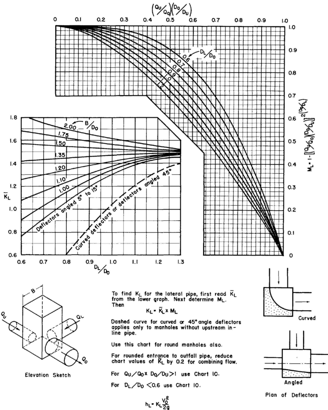
Figure B.8 Chart 8 - Square or Round Manhole At 90° Deflection Or On Through Pipeline At Junction Of 90° Lateral Pipe (Lateral Coefficient) (Source University of Missouri E.S.B. #41)
