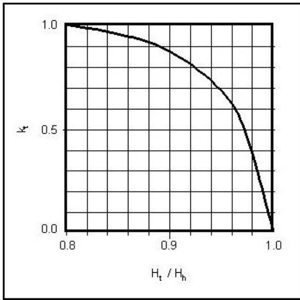
Figure 10.3.13.B - Over-Embarkment Flow Adjustment Factor (Source TxDOT, Hydraulic Design Manual, 2011)
