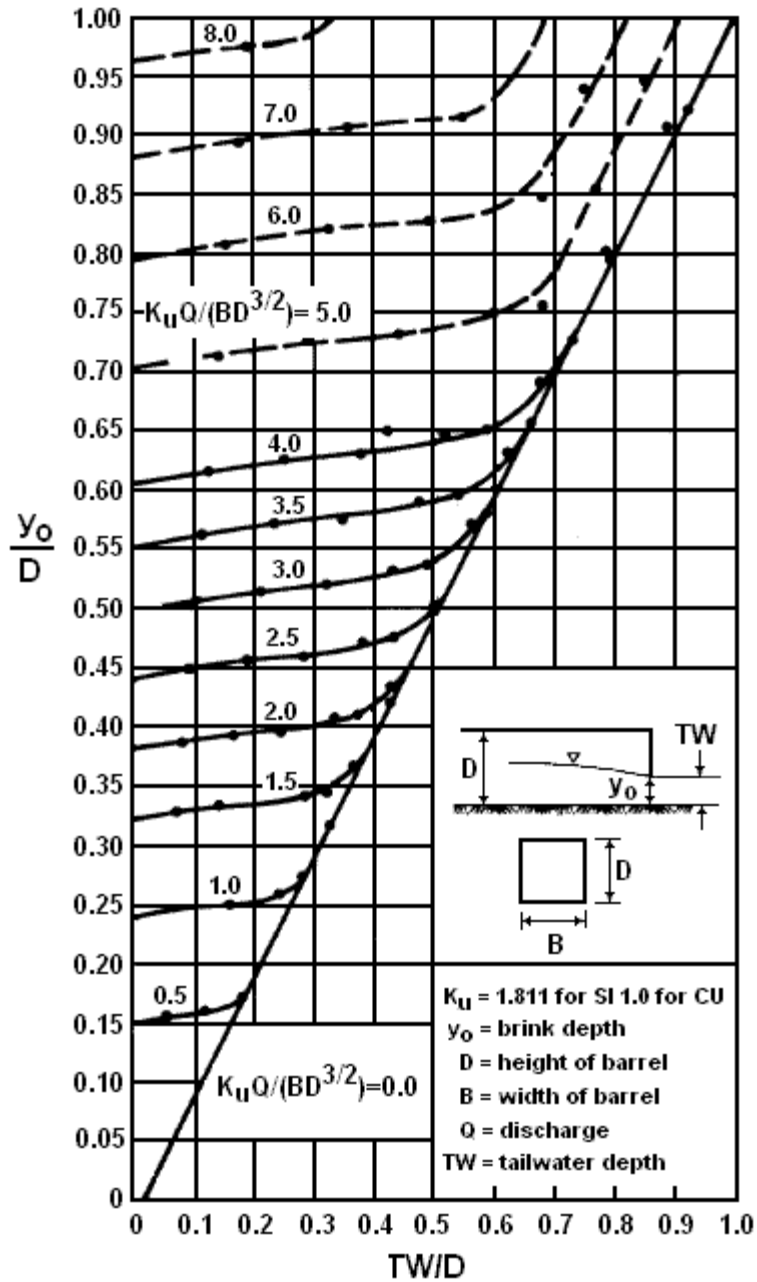
Figure 10.4.3.2.B - Dimensionless Rating Curves for the Outlets of rectangular Culverts on Horizontal and Mild Slopes (Simnos, 1970, Source FHWA, Hydraulic Design of Energy Dissipators for Culverts and Channels , 2006)
