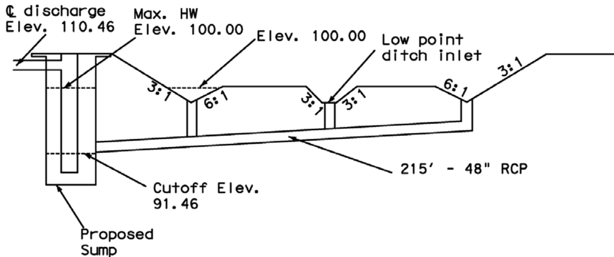
Figure 12.4.1.B - Typical Cross Section (Source TxDOT, Hydraulic Design Manual, 2011)
