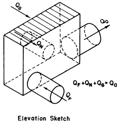
Figure B.7 Chart 7 - Rectangular Inlet With Offset Opposed Lateral Pipes each at 90° To Outfall (With Or Without Grate Flow) (Source University of Missouri E.S.B. #41)
