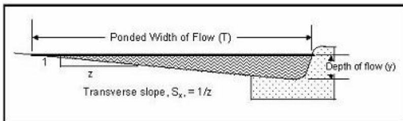
Figure 6.2.1.1 - Gutter Flow (Source TxDOT, 2000)
