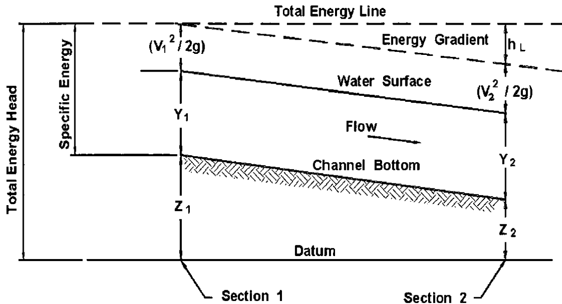
Figure 9.2.1 Total energy in open channels (Source FHWA, HEC-22 Urban Drainage Design Manual, 3ed)
