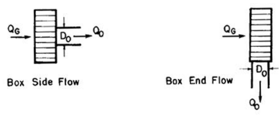
Figure B.2 Chart 2 - Rectangular inlet with grate flow only (Source University of Missouri E.S.B. #41)
