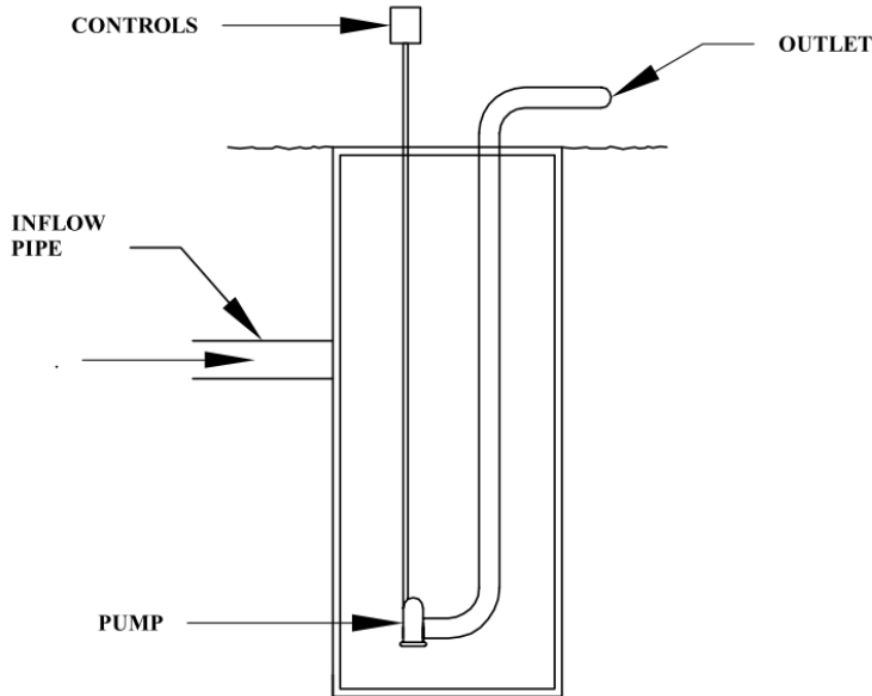
Figure 12.1.1.B - Wet Well
