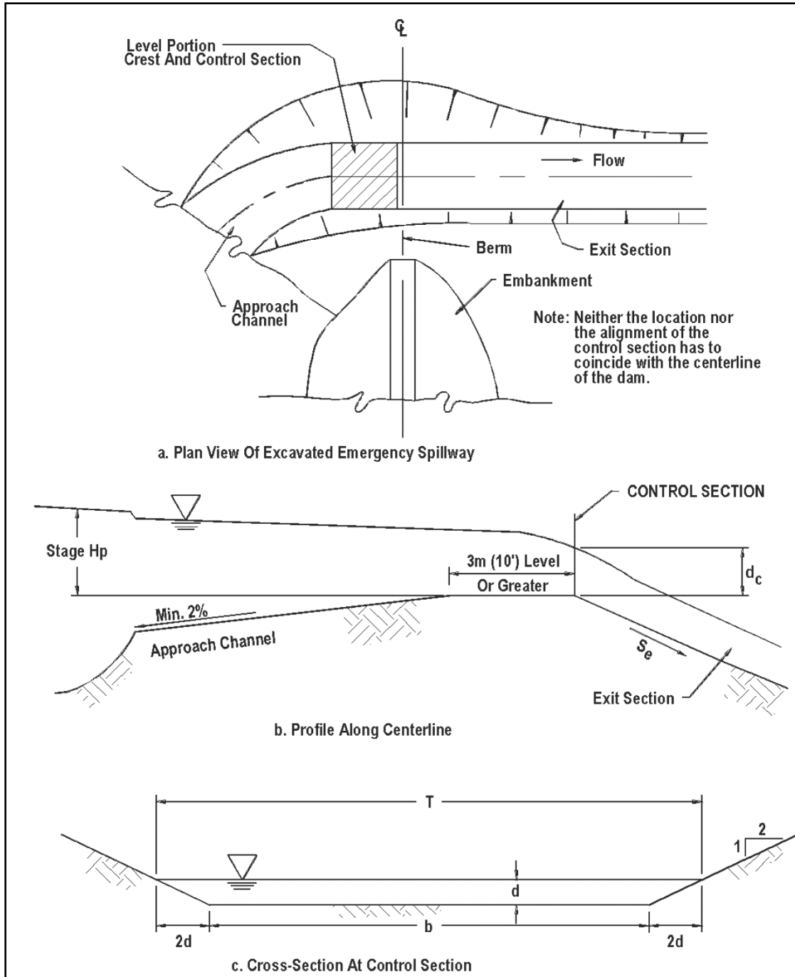
Figure 13.3.2.8a - Auxiliary/Emergency Design Schematic (Source FWA, Urban Drainage Design Manual, Sept. 2009)
