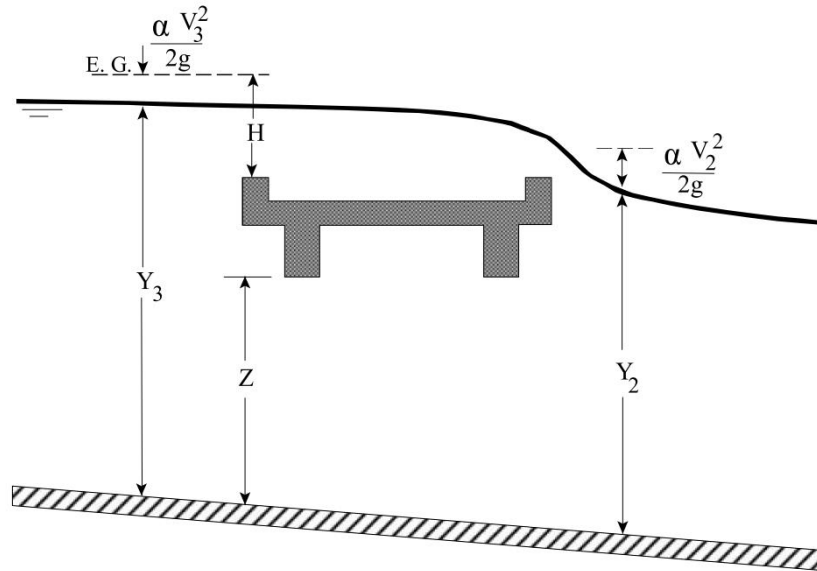
Figure 11.2.2.2.C - Pressure and Weir Flow (Source USACE HEC-RAS Reference Manual)
