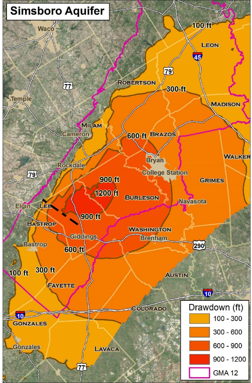
GAM Prediction of Simsboro Drawdowns Due to Baseline plus Vista Ridge, End Op, Forestar, and LCRA Pumping, 2060
