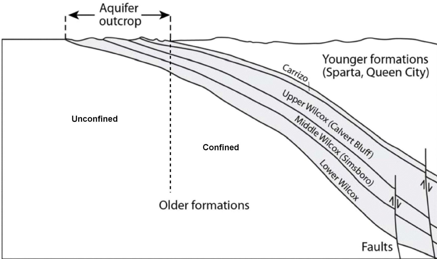
Carrizo-Wilcox Aquifer, Cross Section
