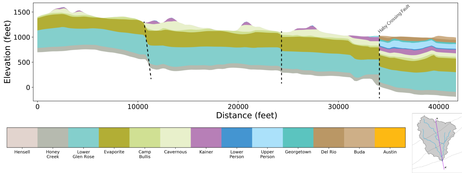
Figure 2-5 Cross section of HSUs within the Helotes Creek watershed. Vertical exaggeration = 5x.
