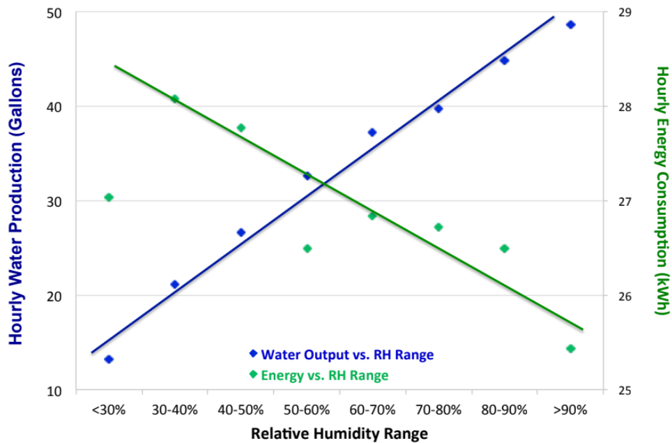
AWG500 hourly energy consumption and water production rates associated with relative humidity over the period of June 4 – August 6, 2015 in San Antonio, TX. Graphic from “Air to Water Technology: AWGTechnology AQ5000 Atmospheric Water Generation (AWG) Unit Performance and Operations Assessment”. 12
